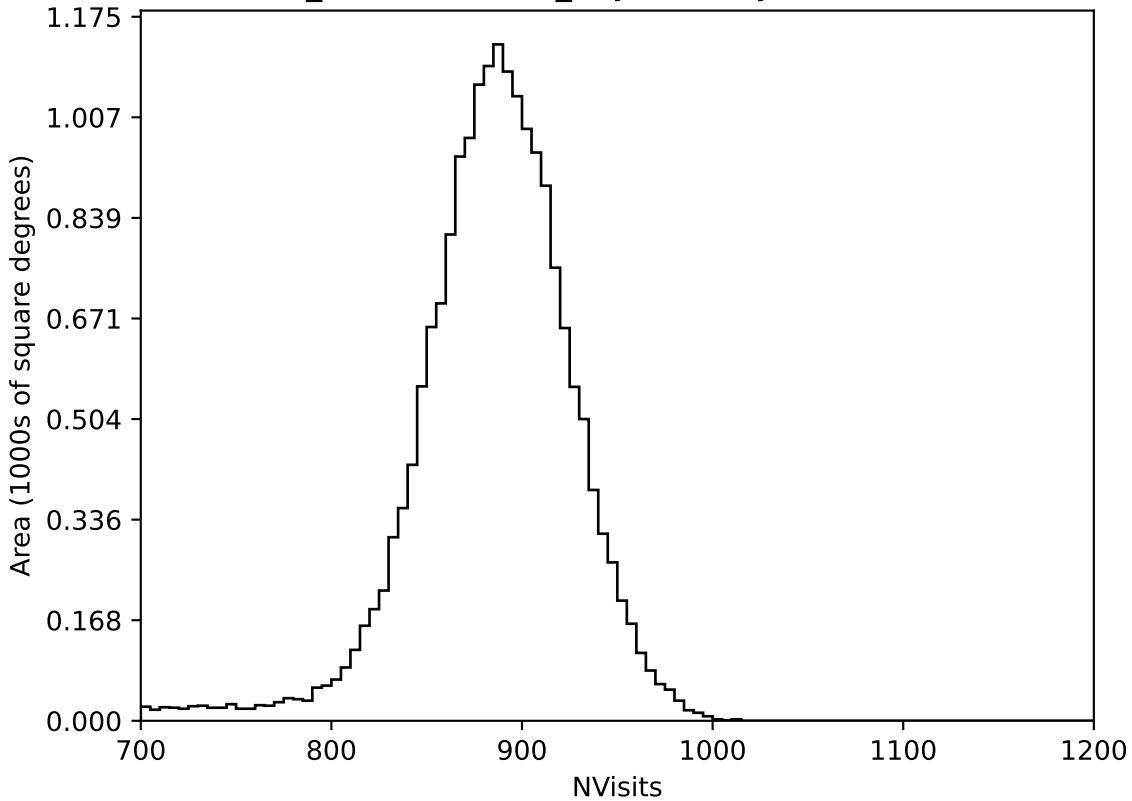
weather_cloudso14v3.4_10yrs All sky all bands: NVisits
