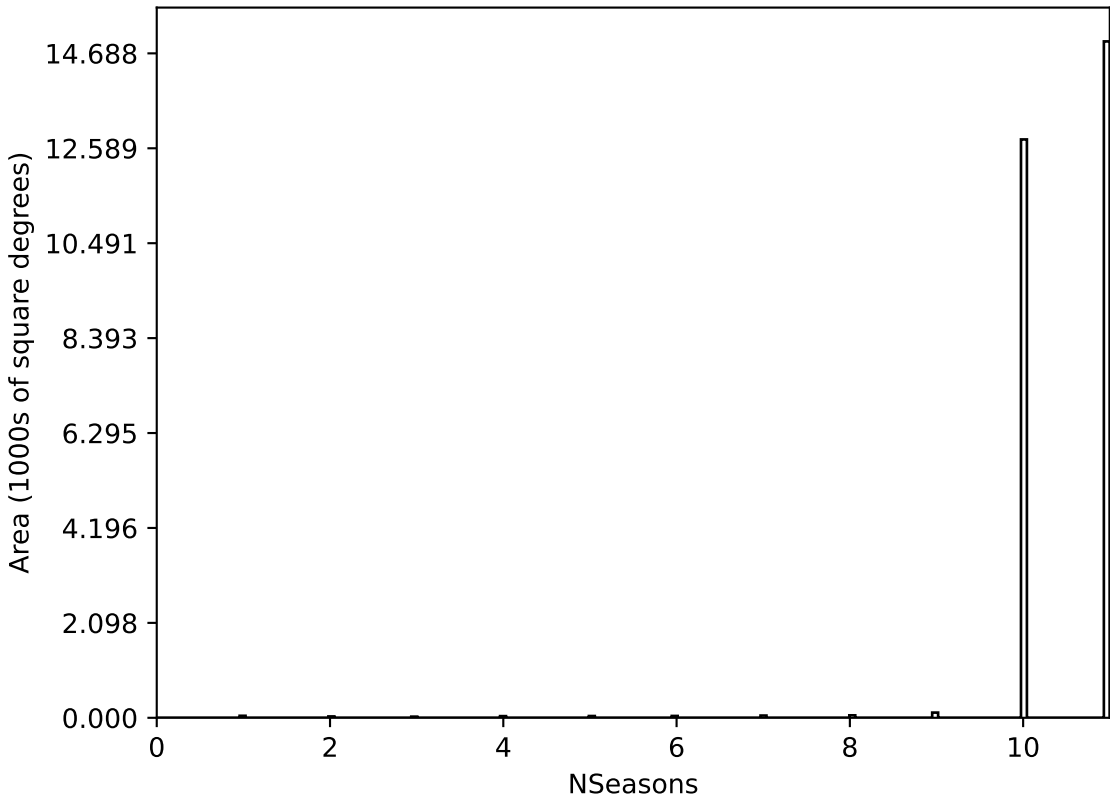
weather_cloudso14v3.4_10yrs All sky all bands: NSeasons
