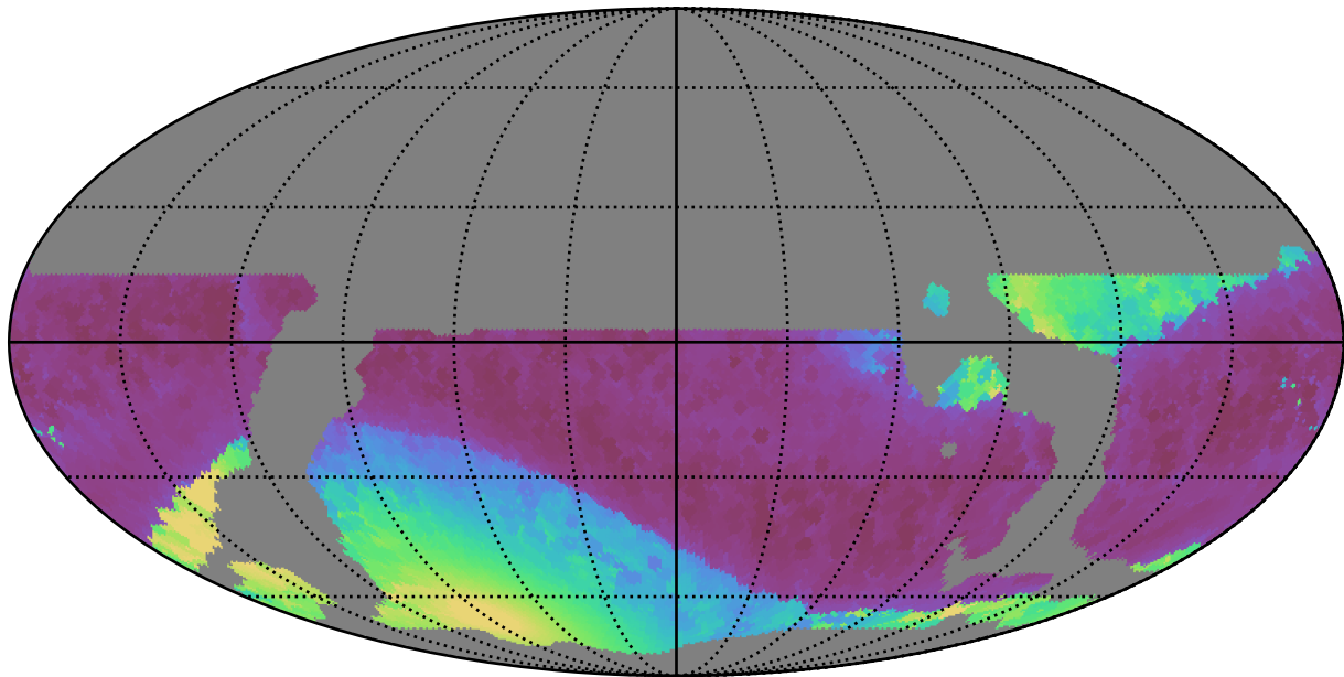
weather_cloudso14v3.4_10yrs WFD all bands: Min solarElong
