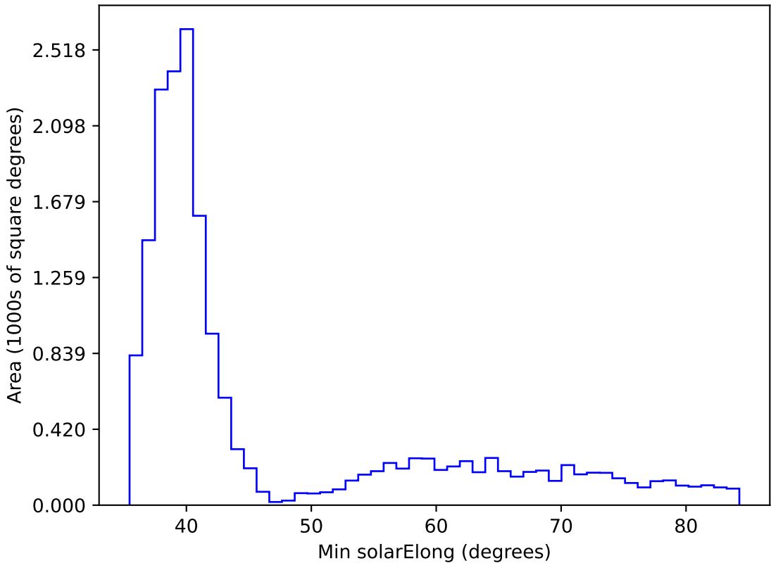
weather_cloudso14v3.4_10yrs WFD all bands: Min solarElong
