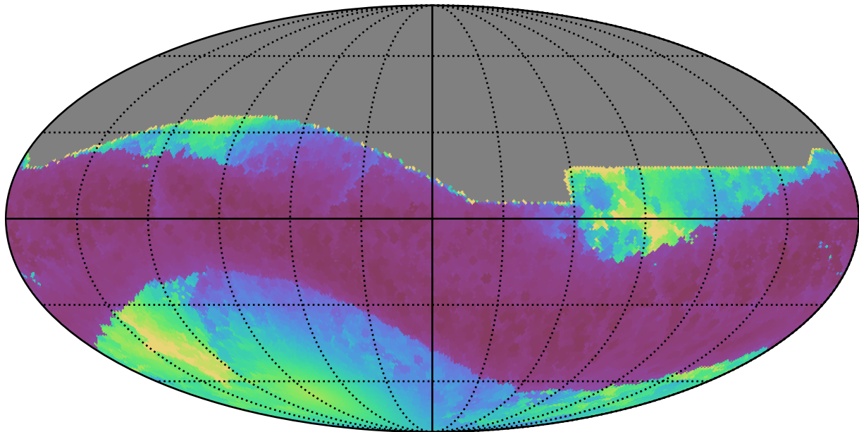
weather_cloudso14v3.4_10yrs All sky all bands: Min solarElong
