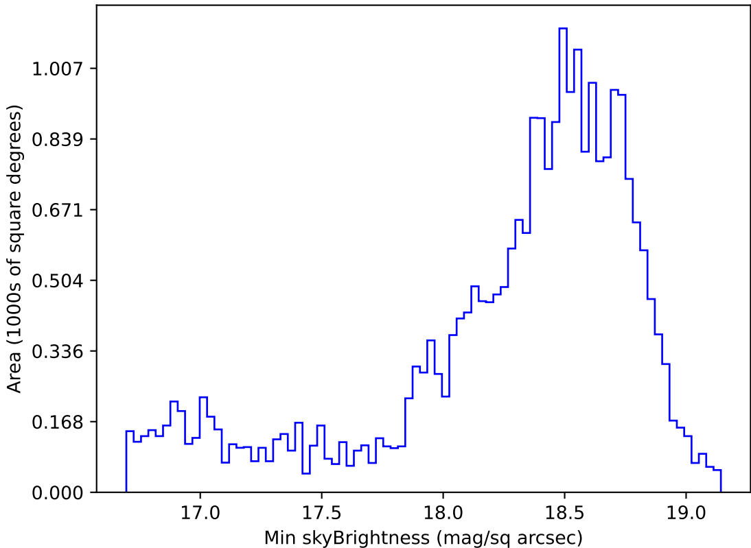
weather_cloudso14v3.4_10yrs Yr 1 z band: Min skyBrightness
