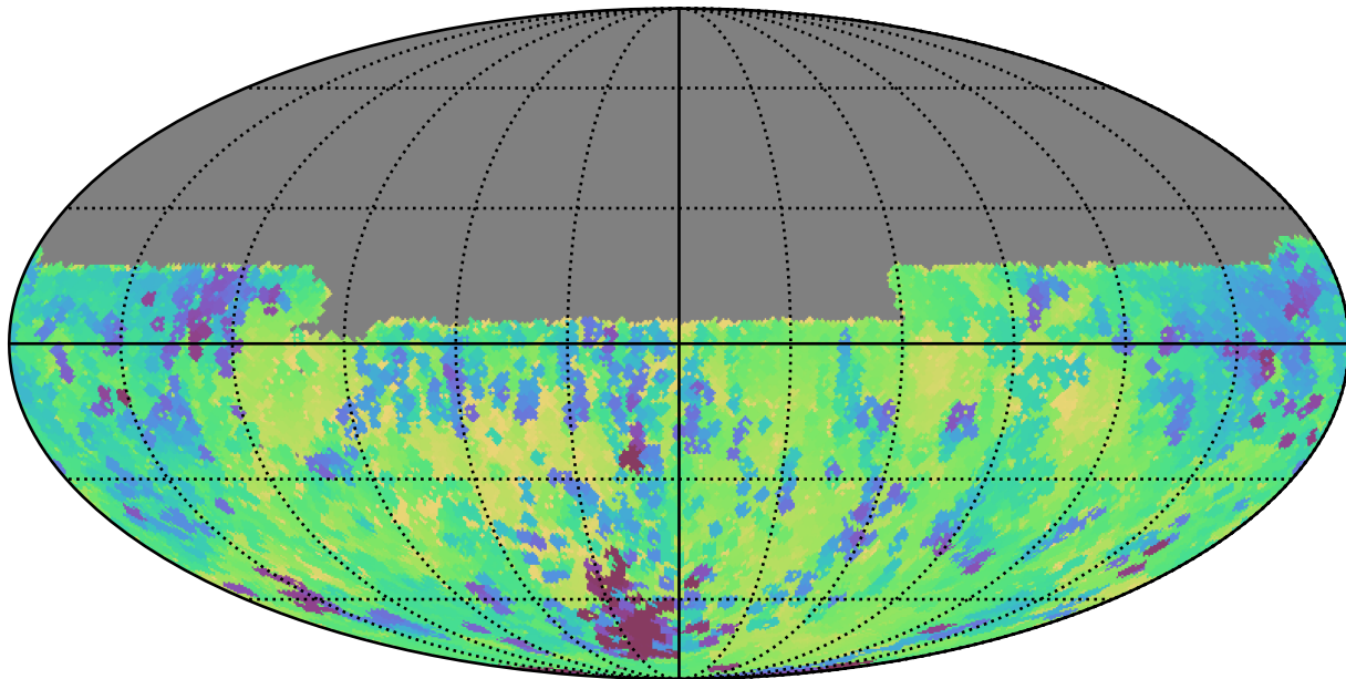
weather_cloudso14v3.4_10yrs Yr 1 y band: Min skyBrightness
