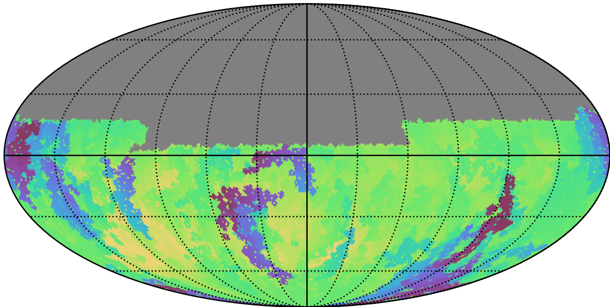
weather_cloudso14v3.4_10yrs Yr 1 u band: Min skyBrightness
