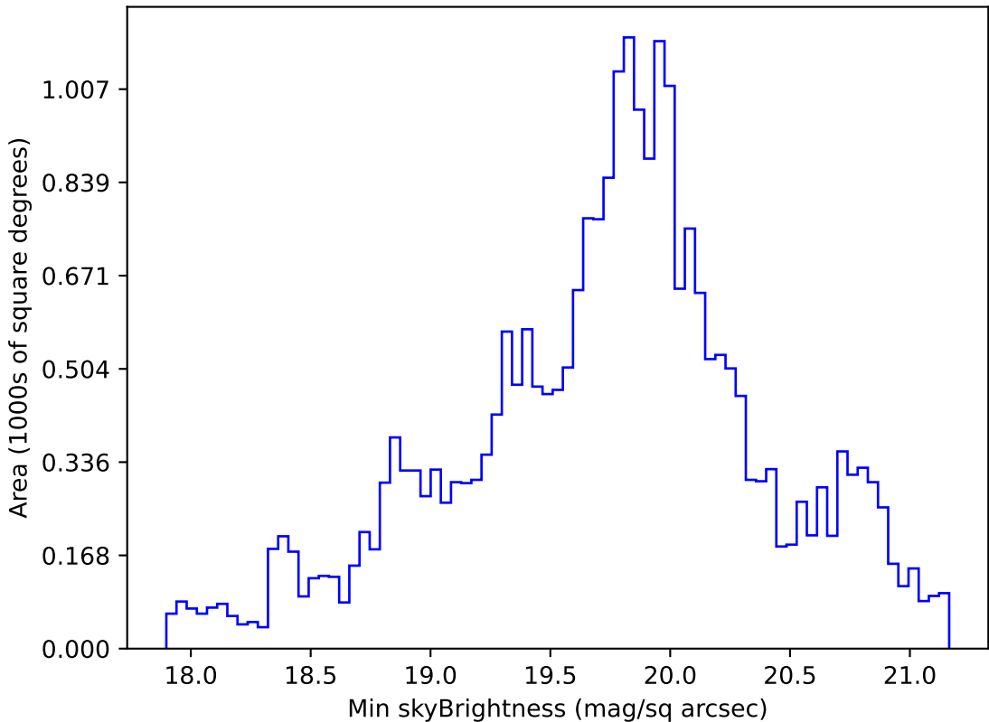
weather_cloudso14v3.4_10yrs Yr 1 r band: Min skyBrightness
