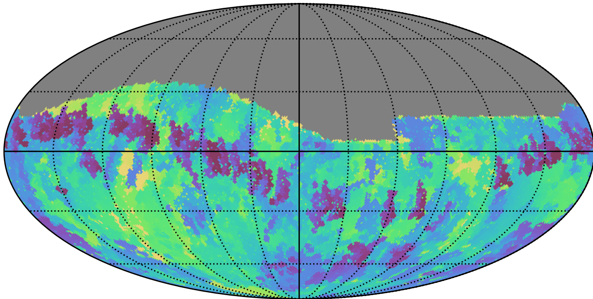
weather_cloudso14v3.4_10yrs Yr 1 i band: Min skyBrightness
