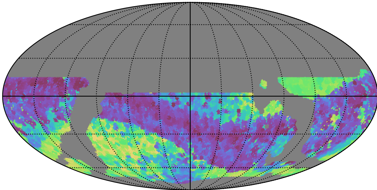
weather_cloudso14v3.4_10yrs WFD z band: Min skyBrightness
