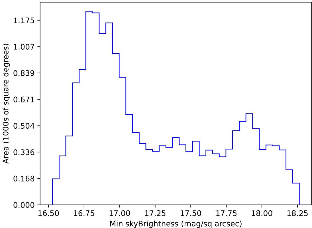
weather_cloudso14v3.4_10yrs WFD z band: Min skyBrightness
