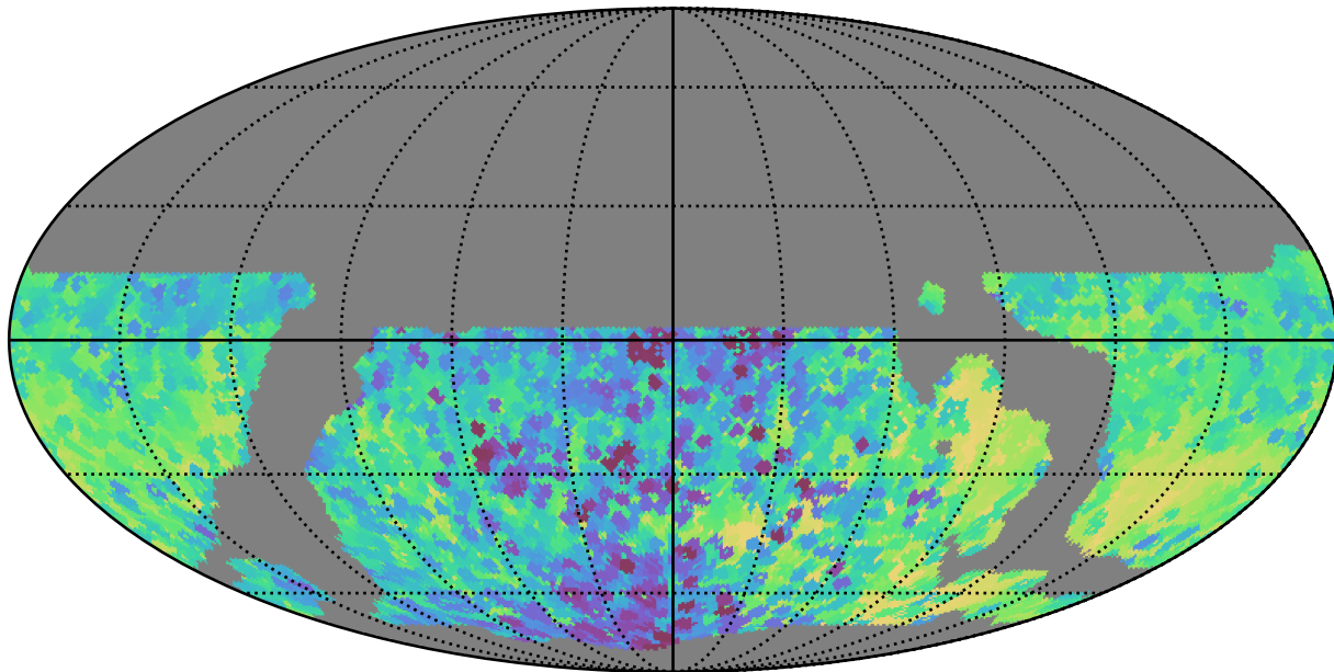
weather_cloudso14v3.4_10yrs WFD y band: Min skyBrightness
