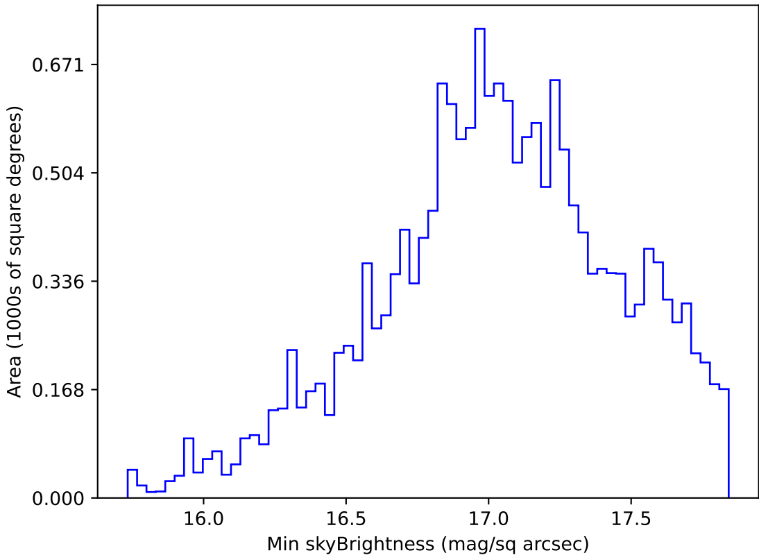
weather_cloudso14v3.4_10yrs WFD y band: Min skyBrightness
