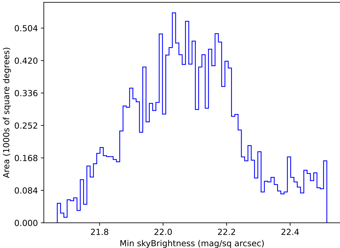
weather_cloudso14v3.4_10yrs WFD u band: Min skyBrightness
