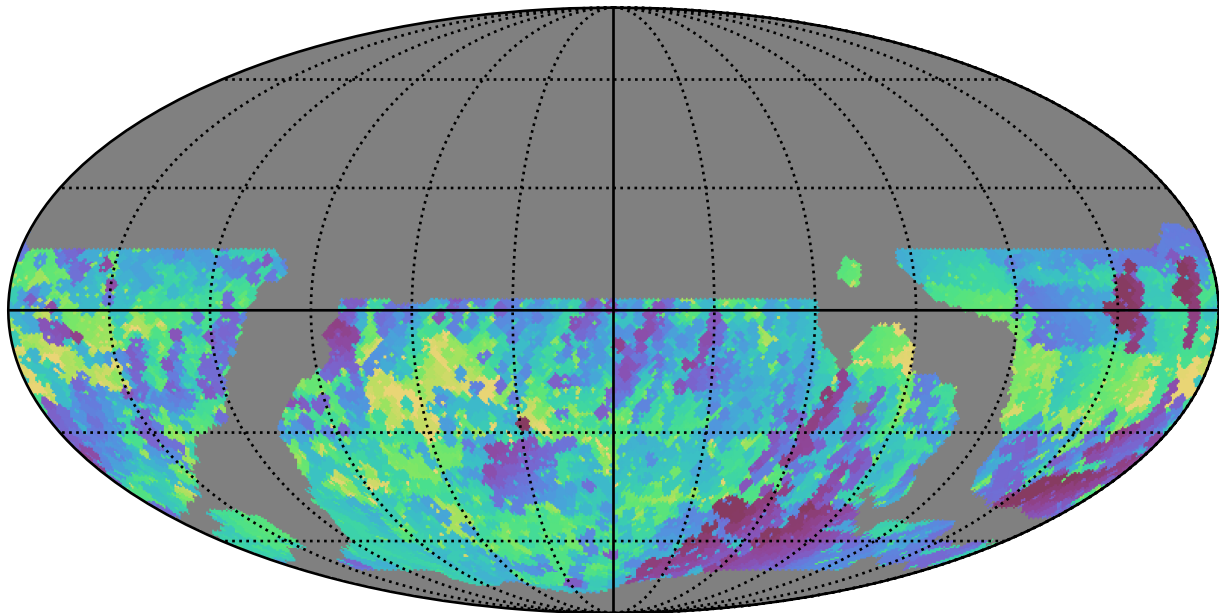
weather_cloudso14v3.4_10yrs WFD r band: Min skyBrightness
