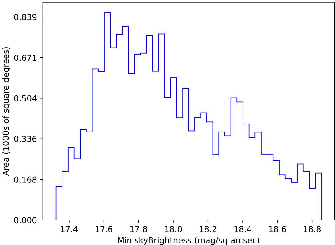
weather_cloudso14v3.4_10yrs WFD i band: Min skyBrightness
