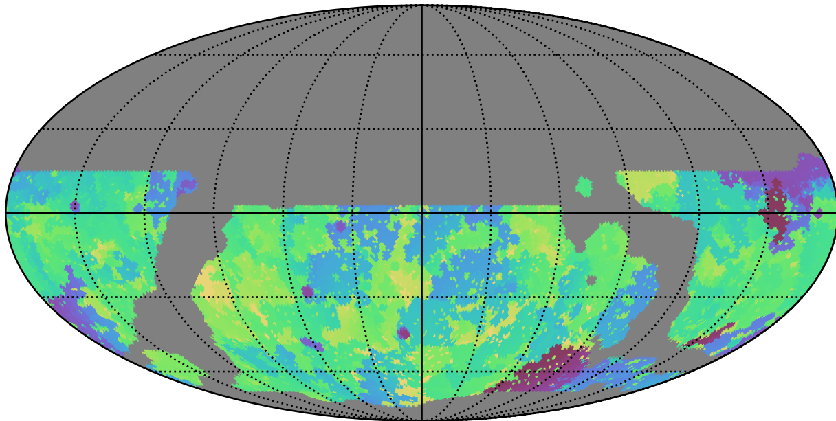
weather_cloudso14v3.4_10yrs WFD g band: Min skyBrightness
