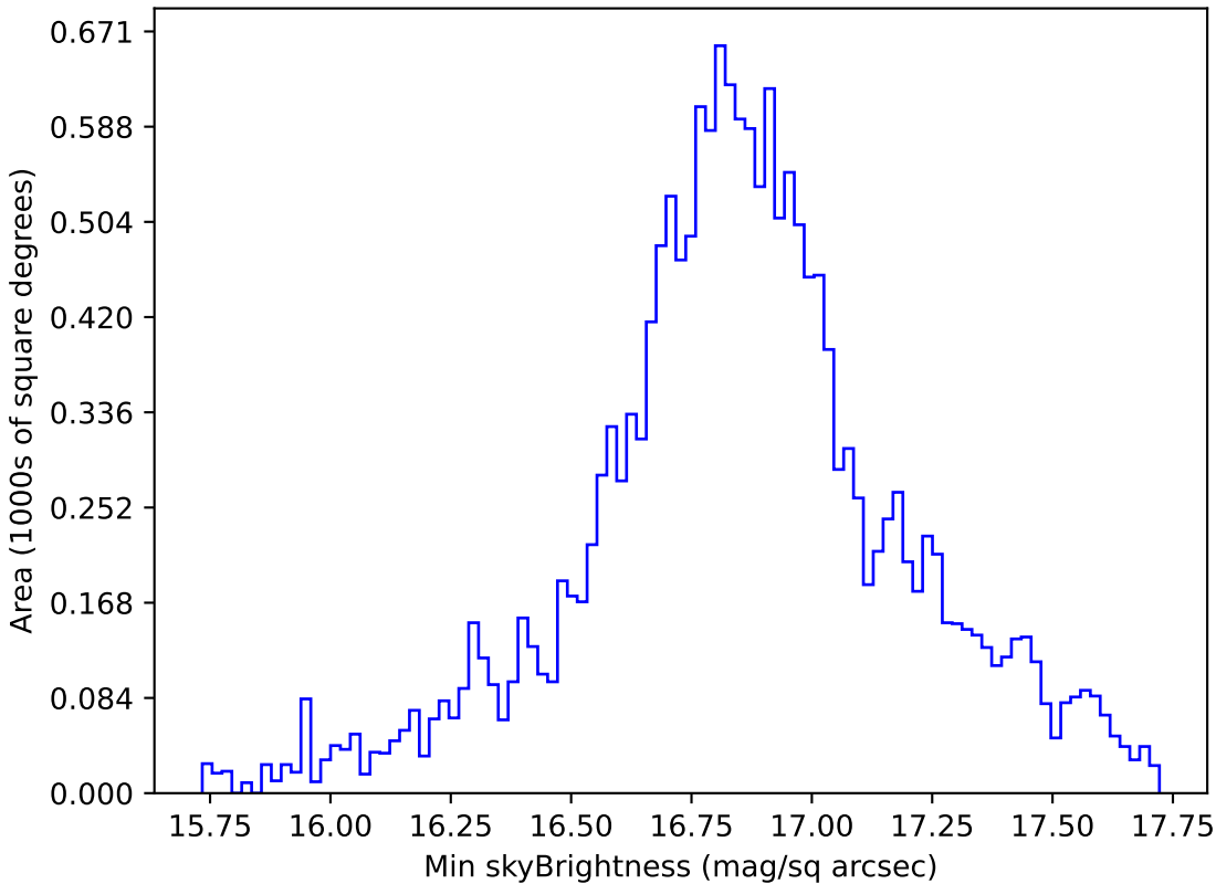
weather_cloudso14v3.4_10yrs WFD all bands: Min skyBrightness
