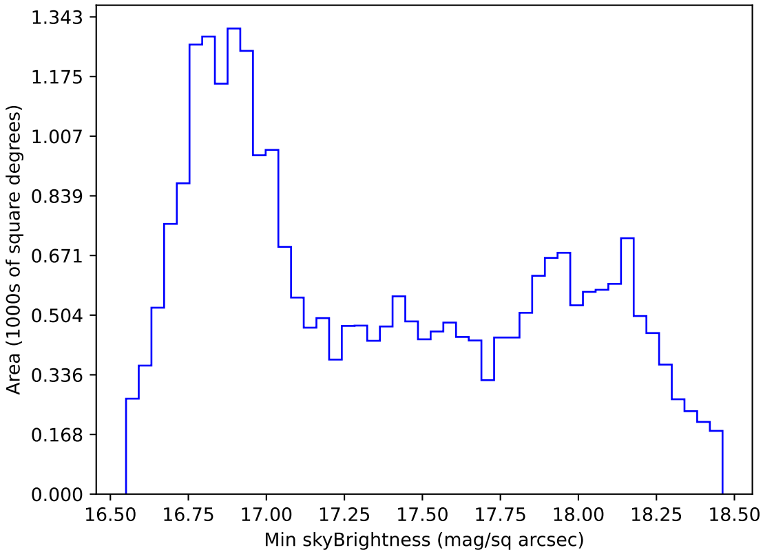
weather_cloudso14v3.4_10yrs All sky z band: Min skyBrightness
