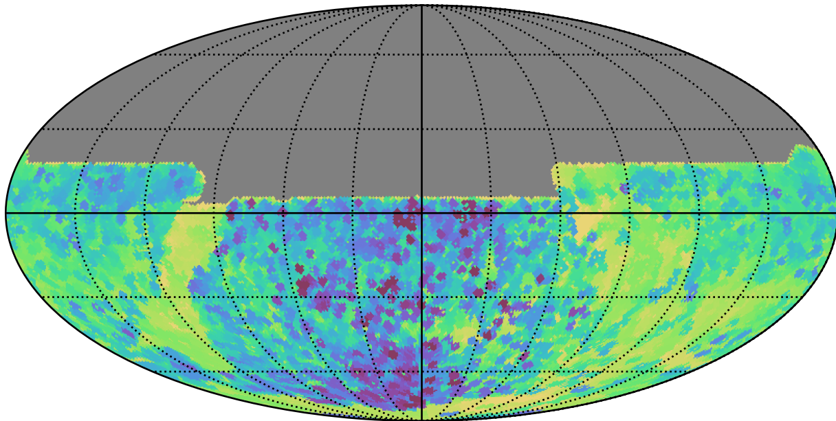
weather_cloudso14v3.4_10yrs All sky y band: Min skyBrightness
