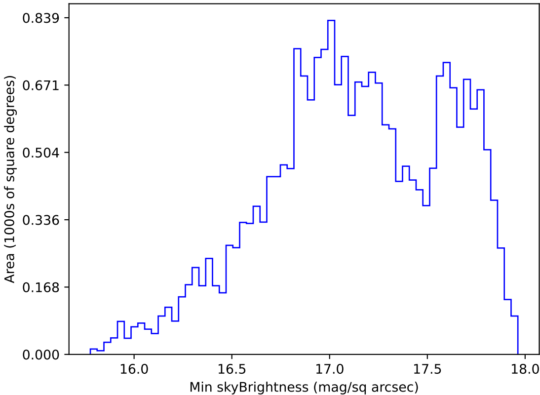
weather_cloudso14v3.4_10yrs All sky y band: Min skyBrightness
