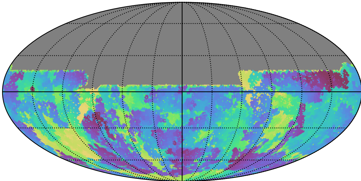
weather_cloudso14v3.4_10yrs All sky u band: Min skyBrightness
