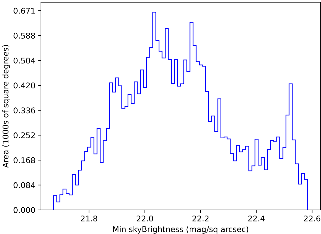
weather_cloudso14v3.4_10yrs All sky u band: Min skyBrightness
