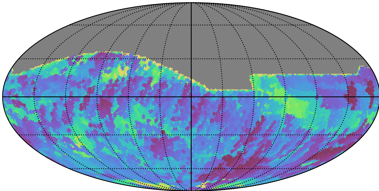
weather_cloudso14v3.4_10yrs All sky r band: Min skyBrightness
