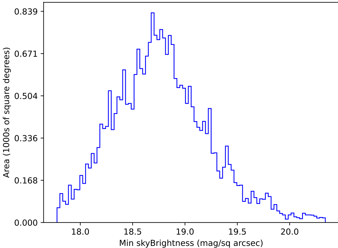
weather_cloudso14v3.4_10yrs All sky r band: Min skyBrightness
