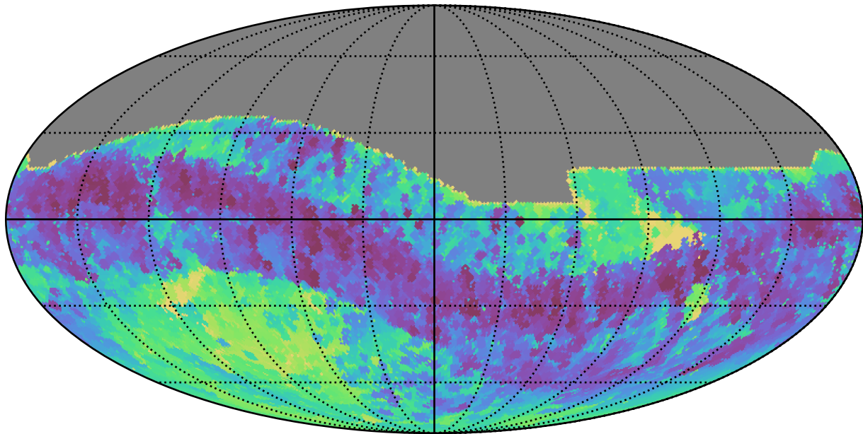
weather_cloudso14v3.4_10yrs All sky i band: Min skyBrightness
