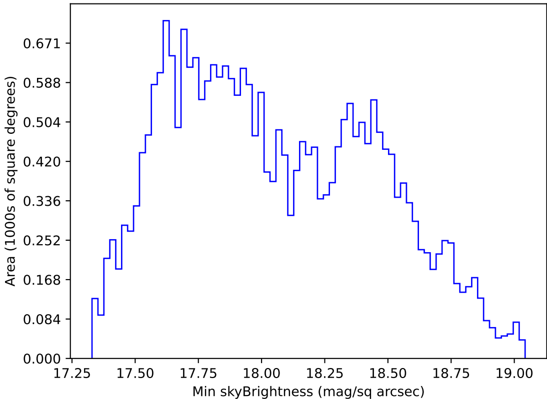
weather_cloudso14v3.4_10yrs All sky i band: Min skyBrightness
