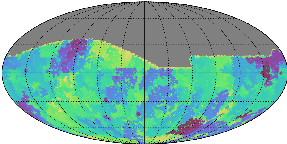
weather_cloudso14v3.4_10yrs All sky g band: Min skyBrightness
