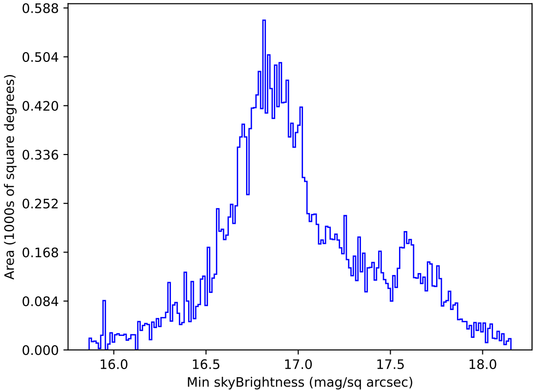
weather_cloudso14v3.4_10yrs All sky all bands: Min skyBrightness
