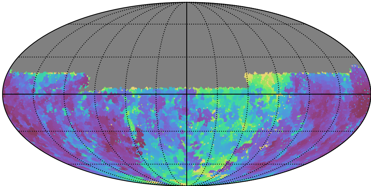
weather_cloudso14v3.4_10yrs Yr 1 u band: Min seeingGeom
