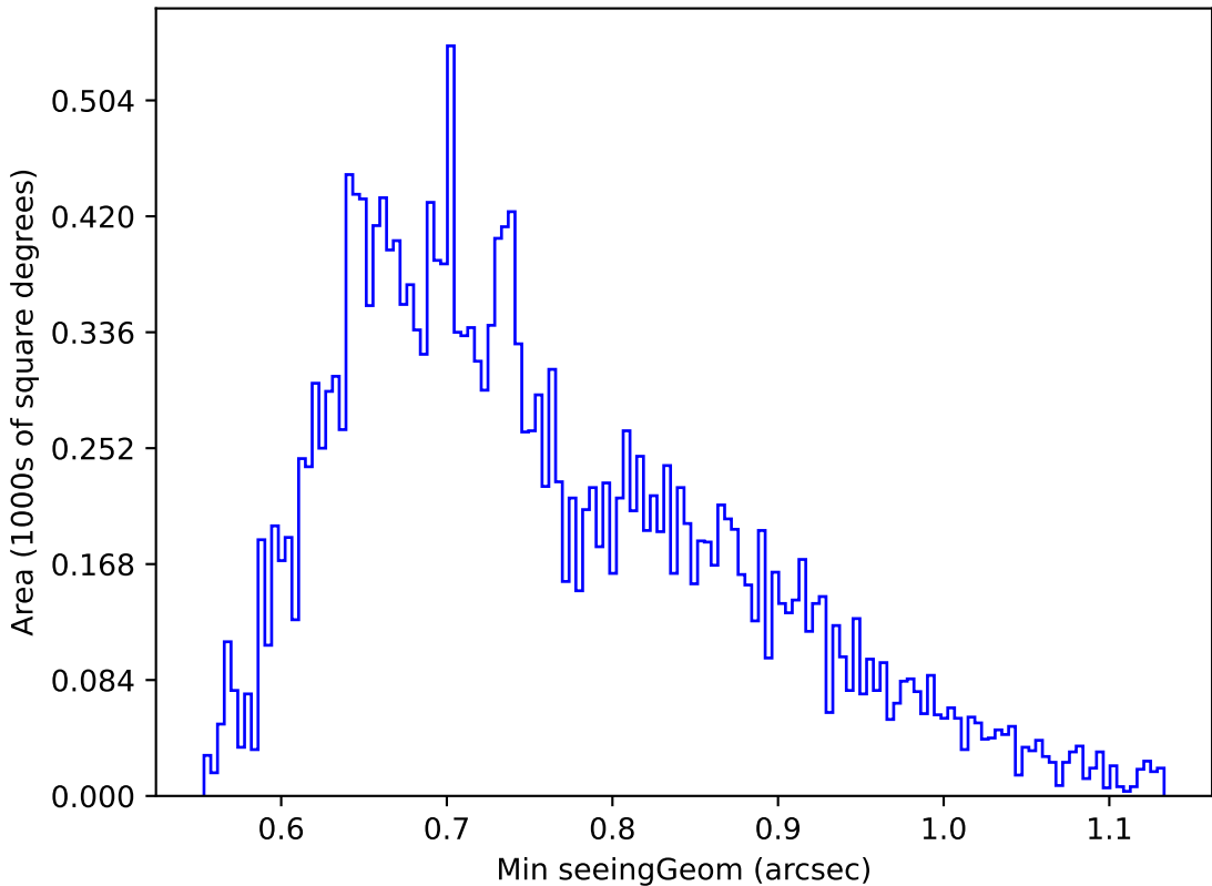
weather_cloudso14v3.4_10yrs Yr 1 u band: Min seeingGeom
