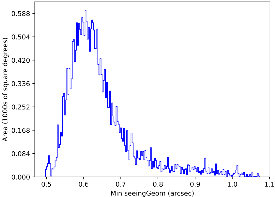
weather_cloudso14v3.4_10yrs Yr 1 r band: Min seeingGeom
