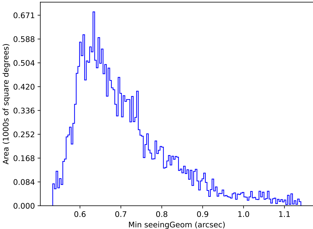
weather_cloudso14v3.4_10yrs Yr 1 g band: Min seeingGeom
