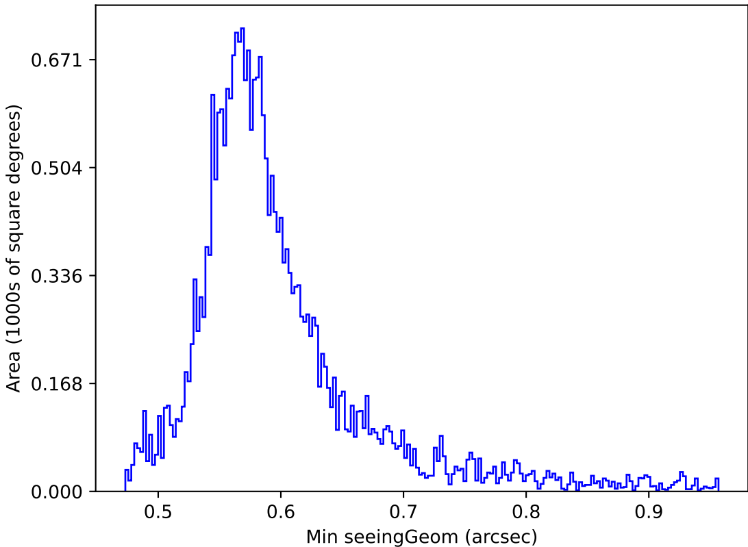
weather_cloudso14v3.4_10yrs Yr 1 all bands: Min seeingGeom
