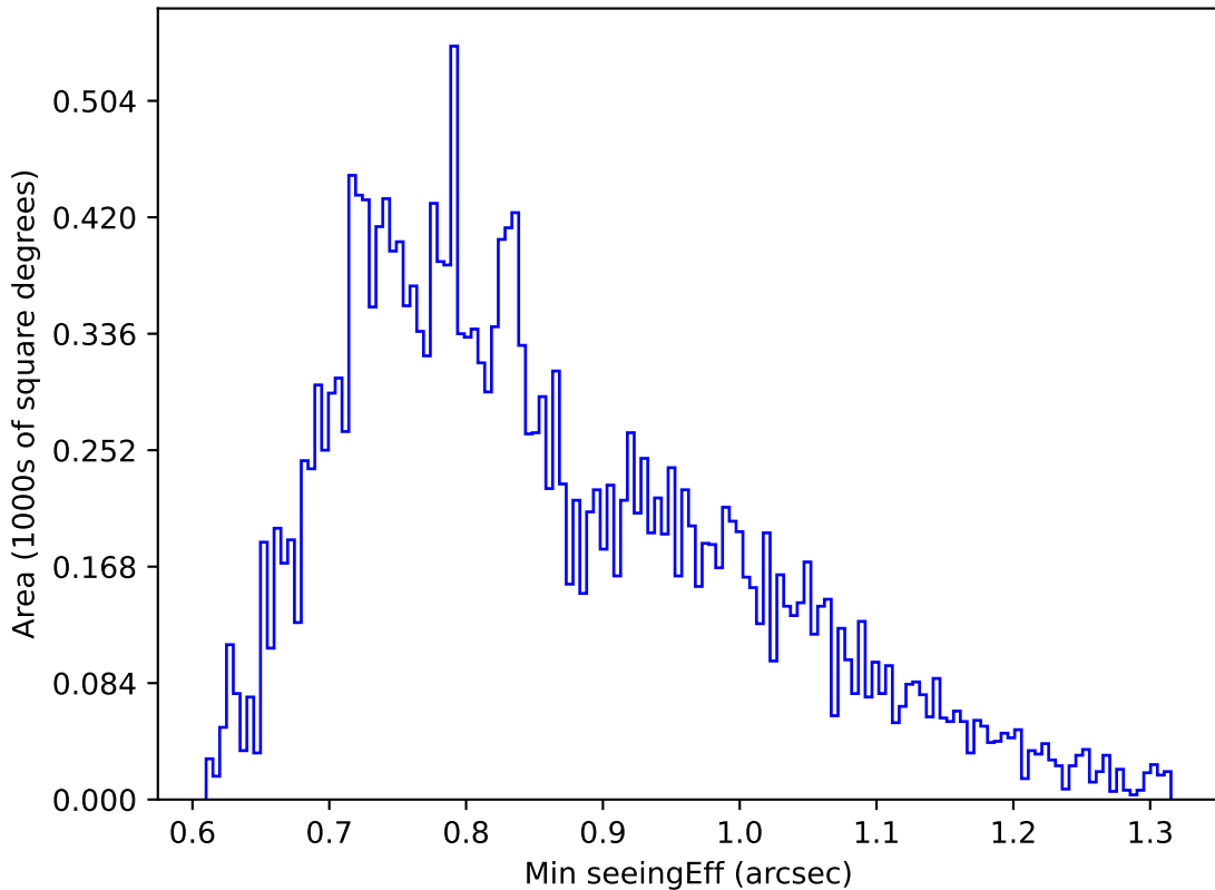
weather_cloudso14v3.4_10yrs Yr 1 u band: Min seeingEff
