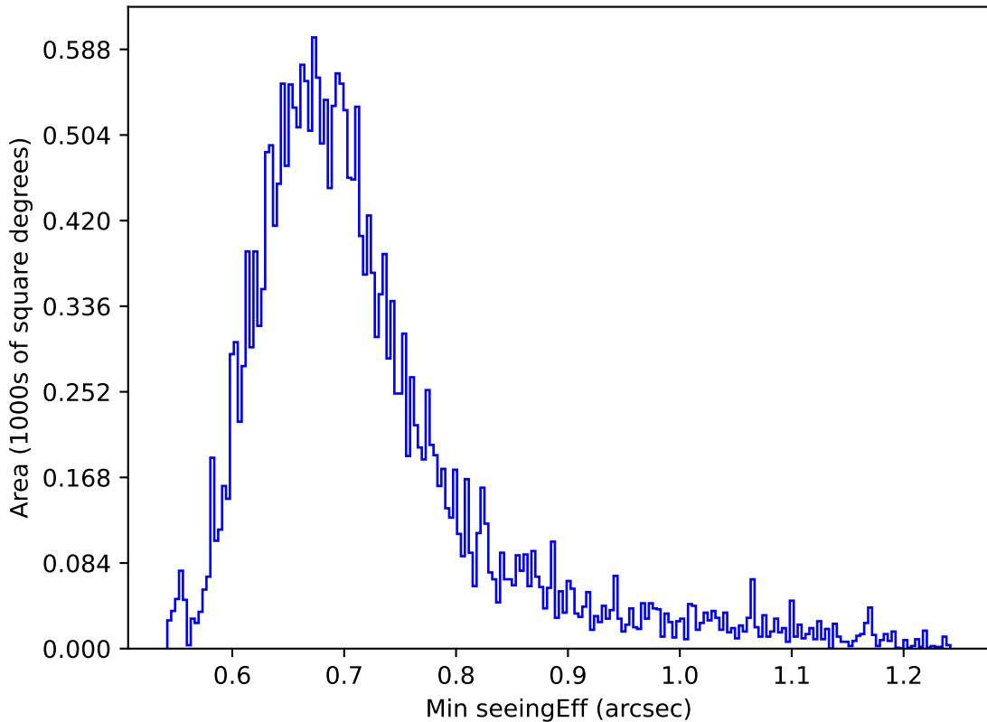
weather_cloudso14v3.4_10yrs Yr 1 r band: Min seeingEff
