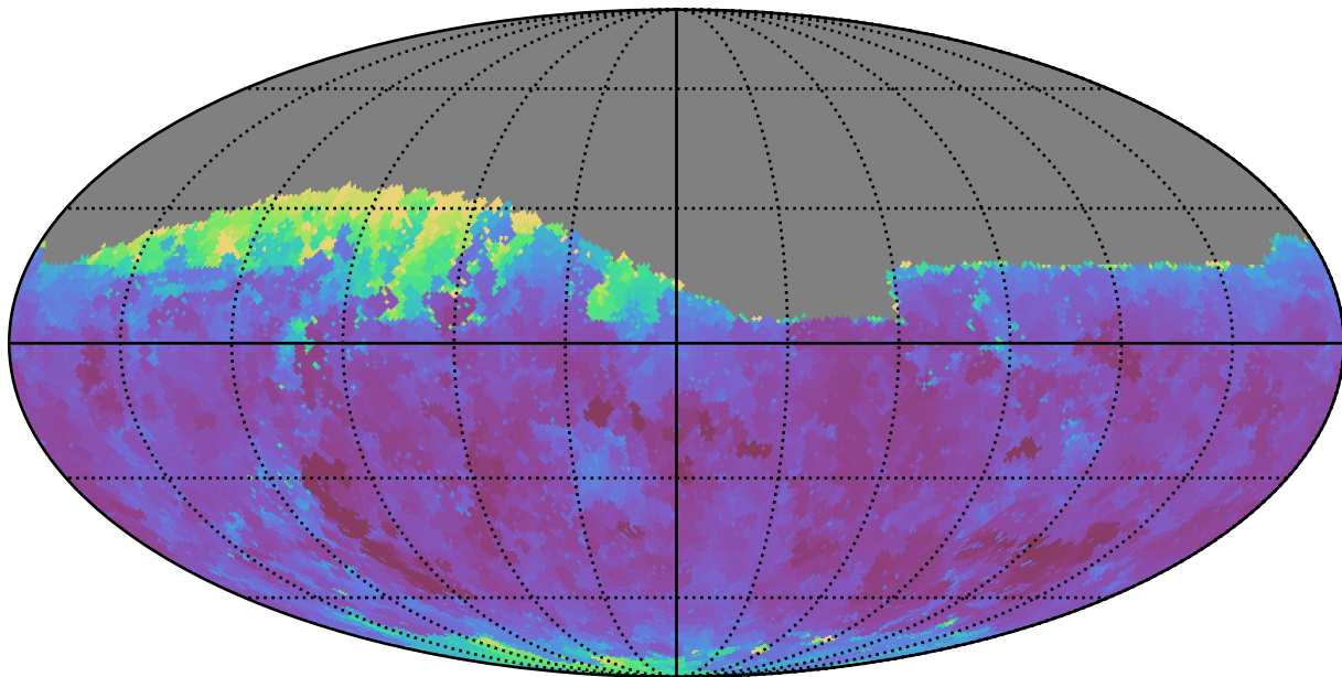
weather_cloudso14v3.4_10yrs Yr 1 i band: Min seeingEff
