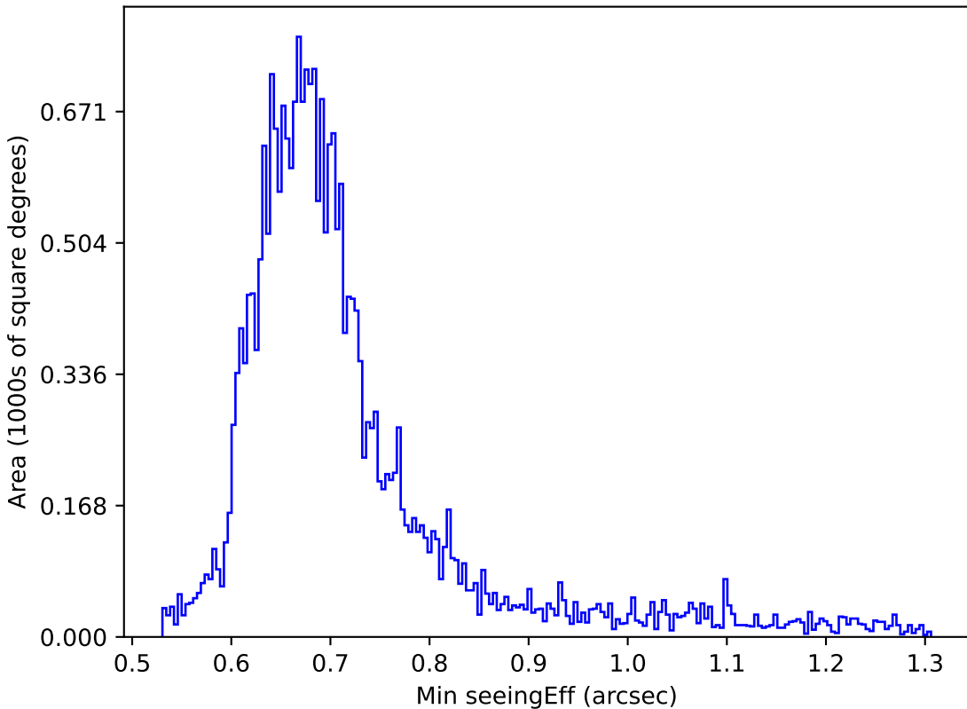
weather_cloudso14v3.4_10yrs Yr 1 i band: Min seeingEff
