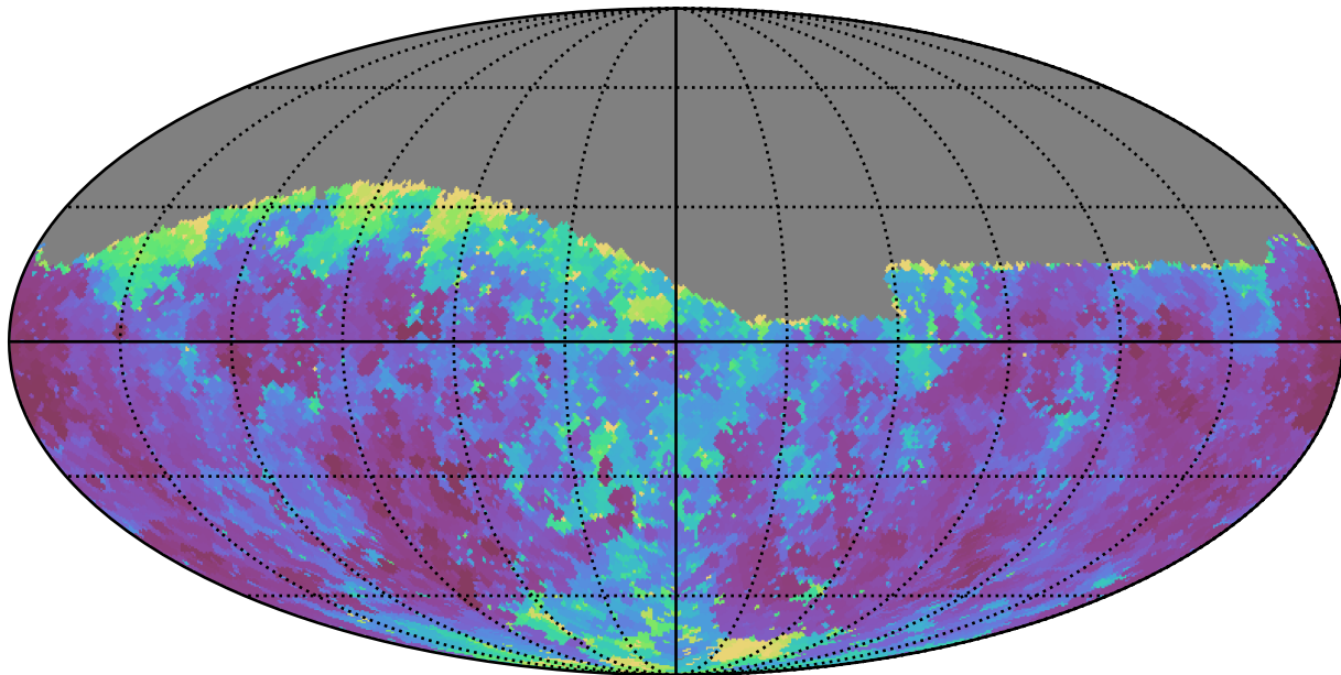
weather_cloudso14v3.4_10yrs Yr 1 g band: Min seeingEff
