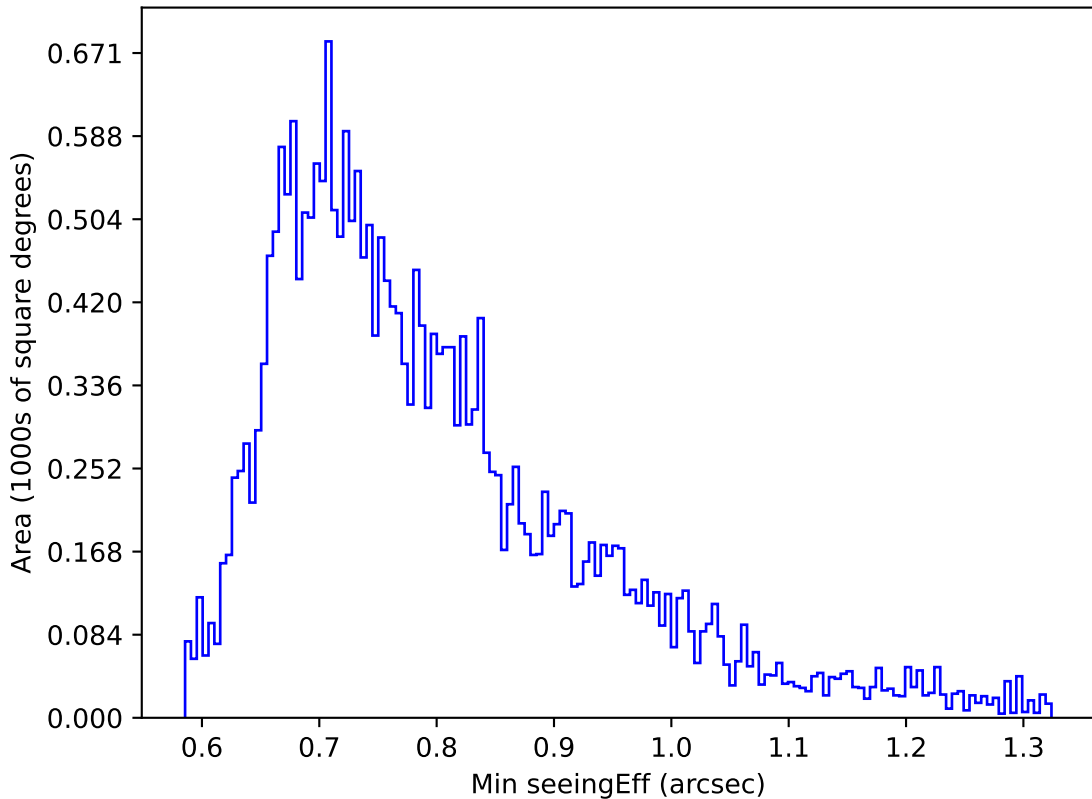
weather_cloudso14v3.4_10yrs Yr 1 g band: Min seeingEff
