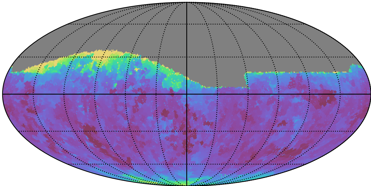
weather_cloudso14v3.4_10yrs Yr 1 all bands: Min seeingEff
