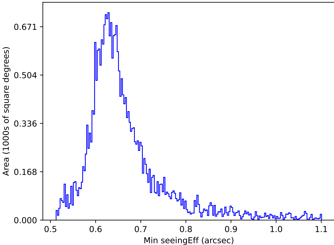
weather_cloudso14v3.4_10yrs Yr 1 all bands: Min seeingEff
