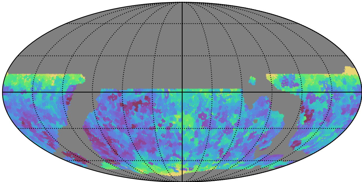
weather_cloudso14v3.4_10yrs WFD z band: Min seeingEff
