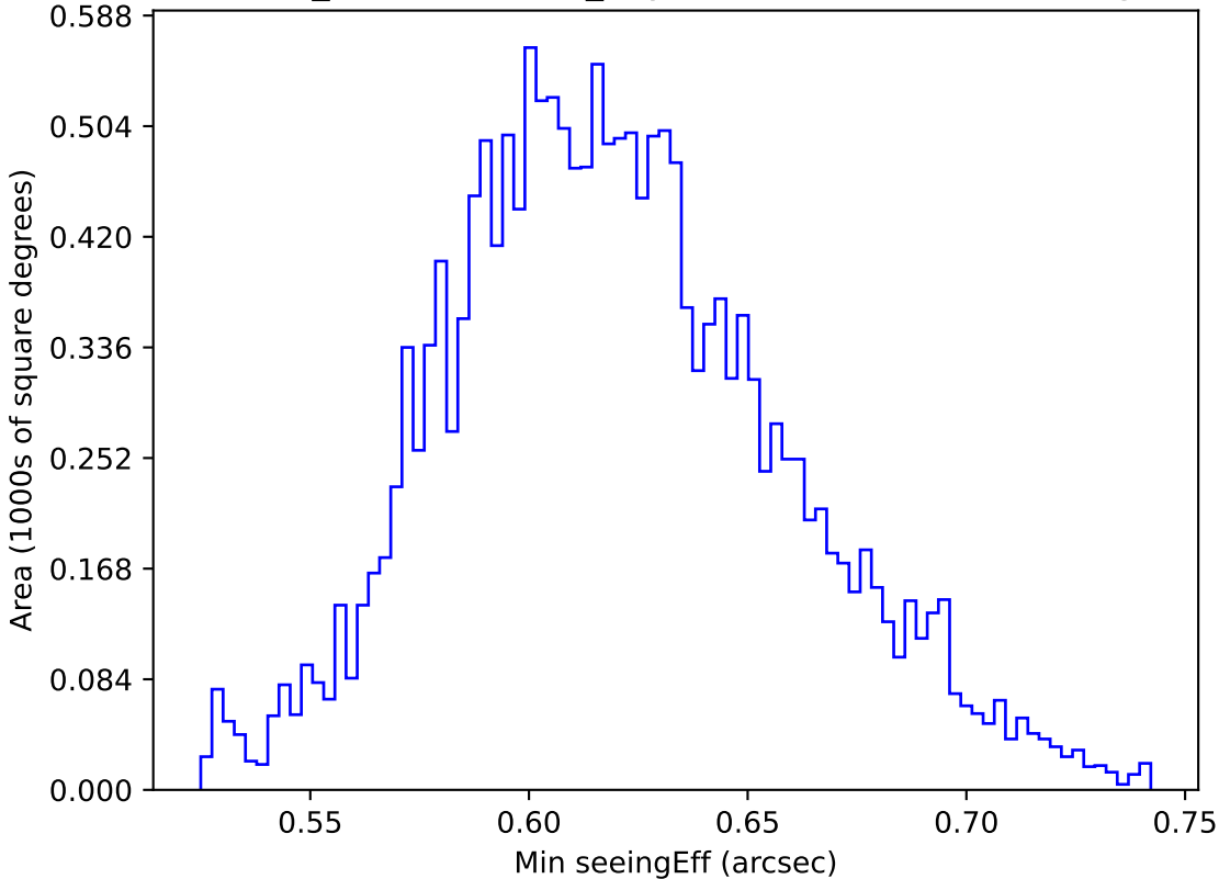
weather_cloudso14v3.4_10yrs WFD z band: Min seeingEff
