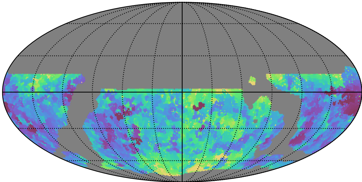
weather_cloudso14v3.4_10yrs WFD u band: Min seeingEff
