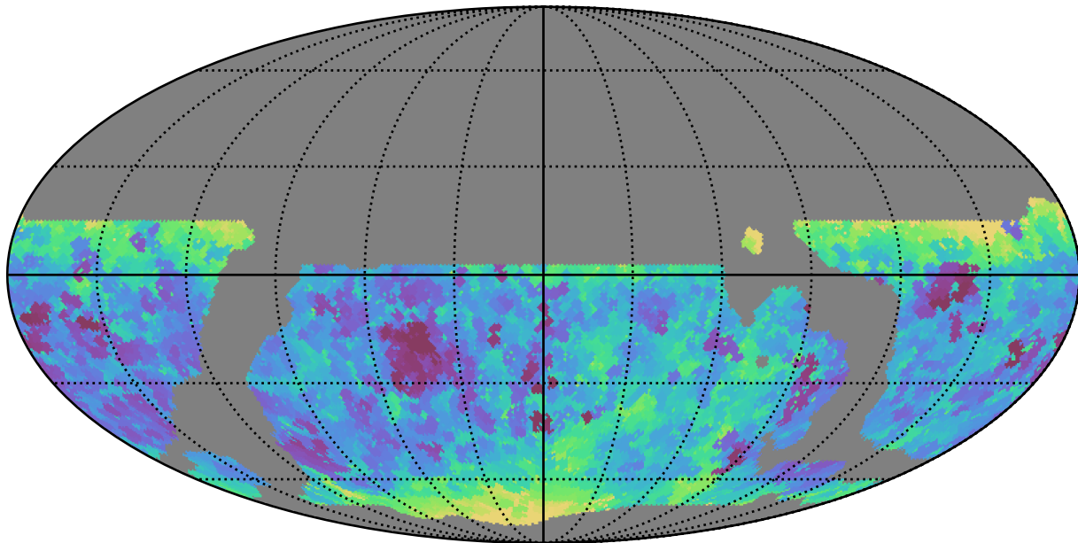
weather_cloudso14v3.4_10yrs WFD r band: Min seeingEff
