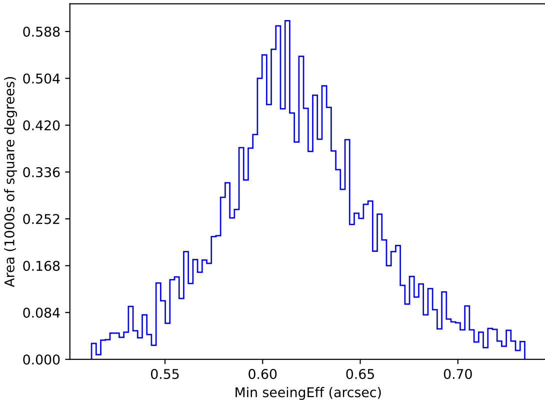
weather_cloudso14v3.4_10yrs WFD r band: Min seeingEff
