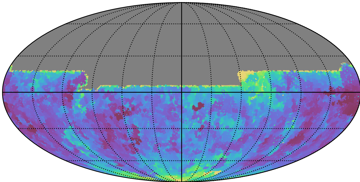
weather_cloudso14v3.4_10yrs All sky u band: Min seeingEff
