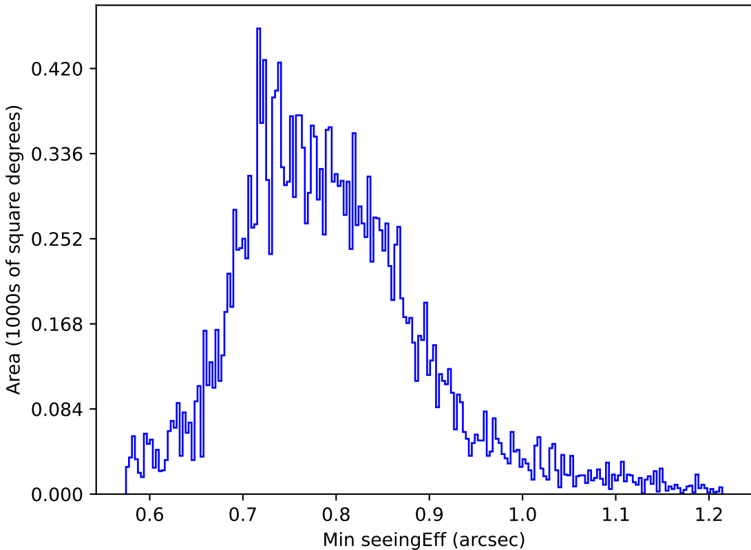
weather_cloudso14v3.4_10yrs All sky u band: Min seeingEff
